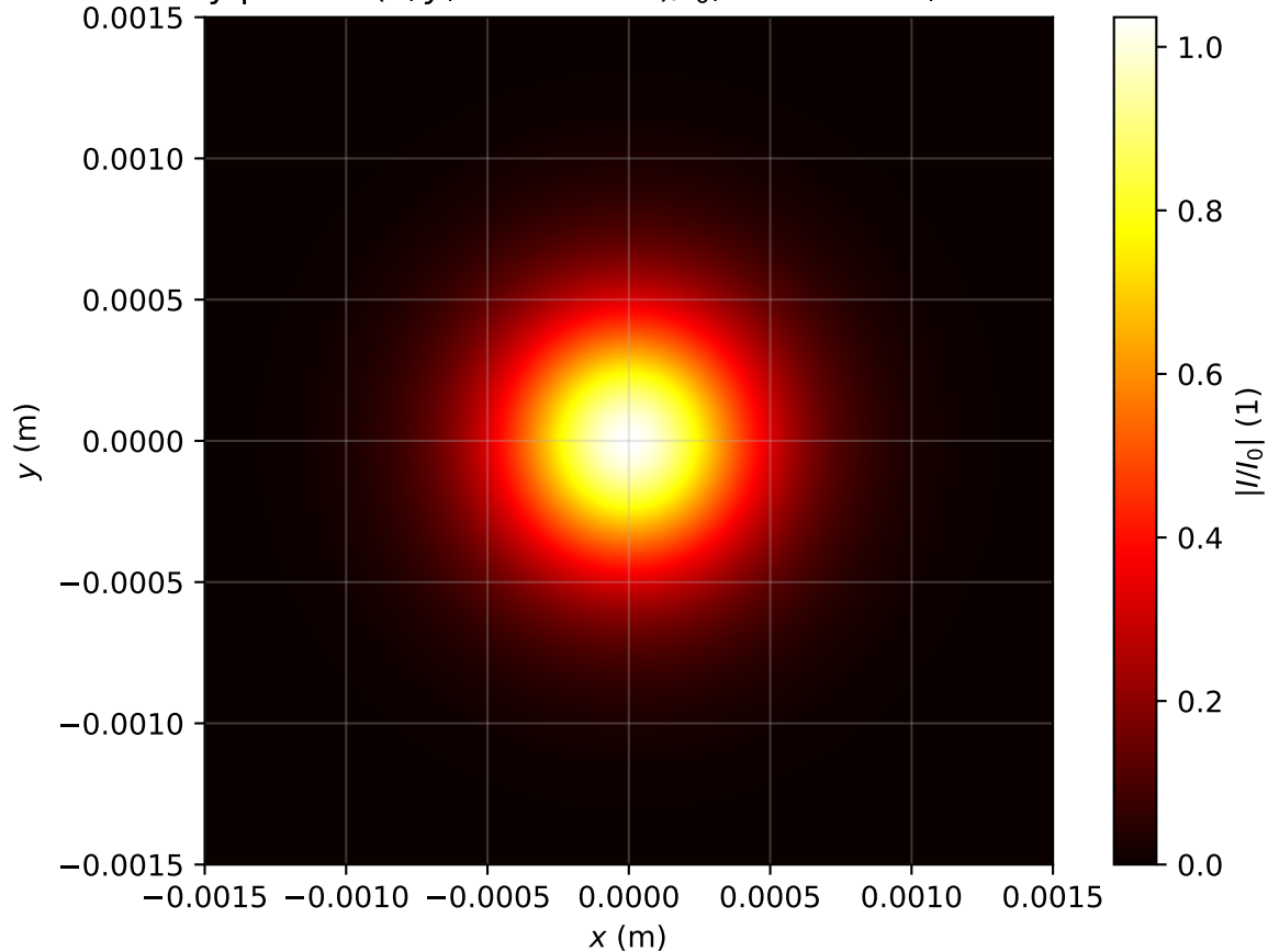
Intensity profile I(x, y, z = 1.115m)/I_0 , \text{Pin}=0.5\text{Pcr} , artificial time
